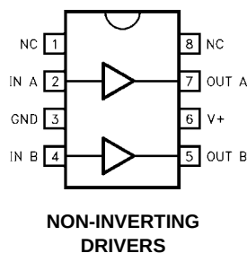
EL7202 (8-PIN PDIP, SO) TOP VIEW
